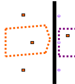
Figure 7 - Best plane bisects the reduced convex hulls
